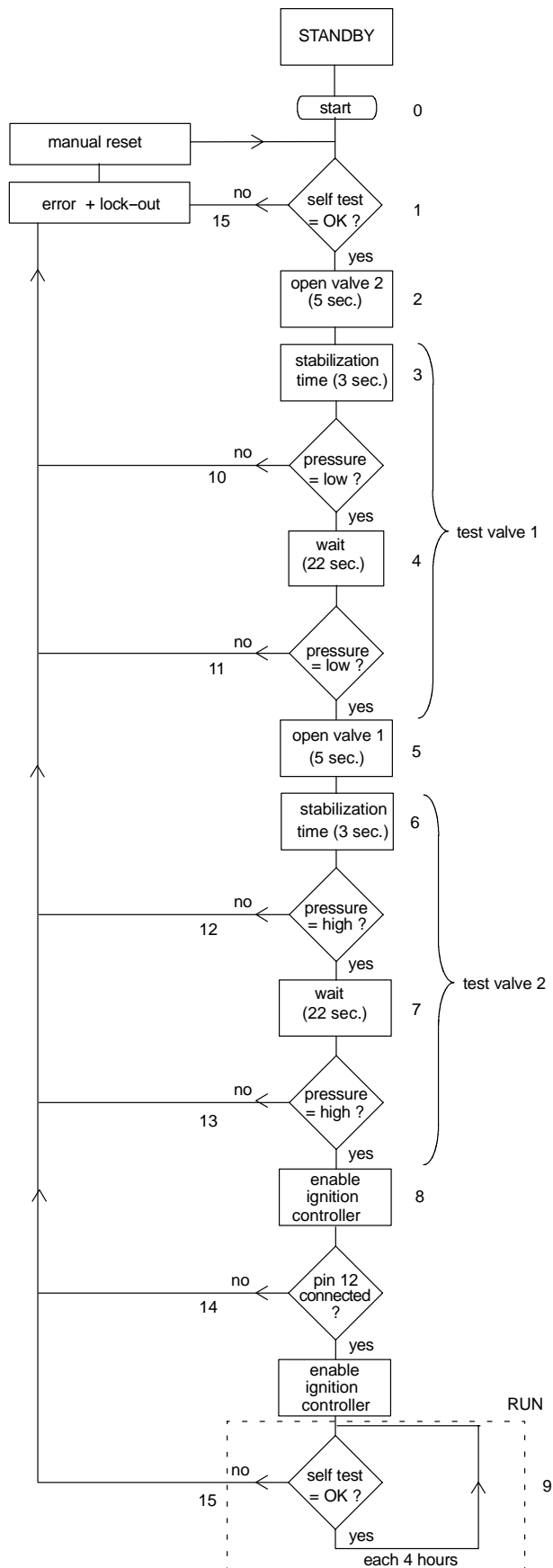
Fig. 5. General flow chart valve proving (given timings for A4021A1002/1010)
