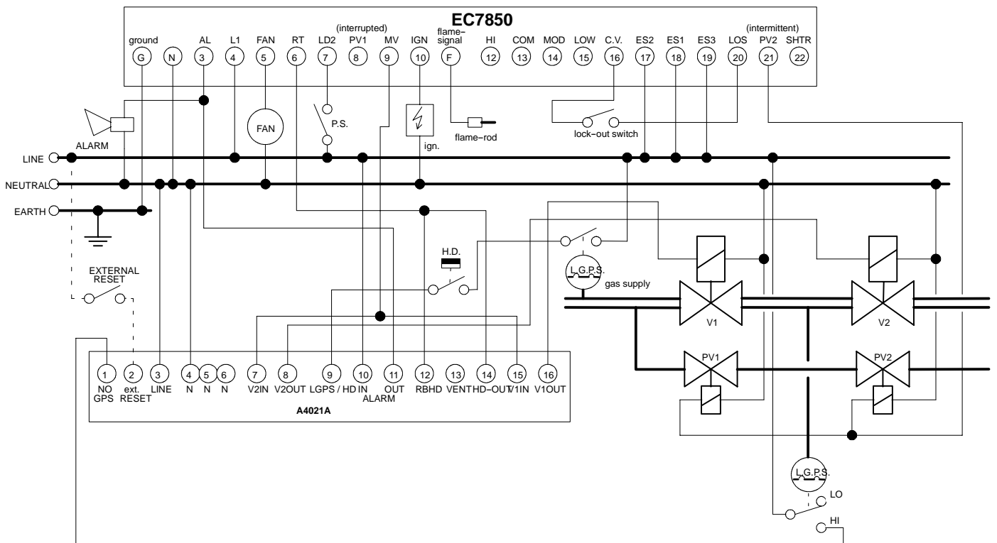
Fig. 15. Wiring diagram A4021A – EC7850: pre-configuration, intermittent pilot, 4-valve configuration
