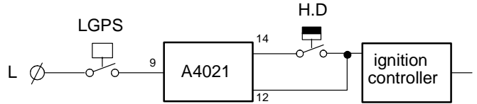
Fig. 3. Valve proving post-configuration .
