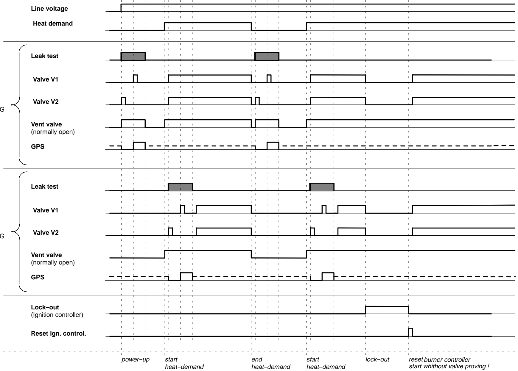
Fig. 6. System sequence of A4021A in post and pre-configuration.
