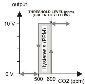
Fig. 4. Relay output (digital) of pin 2
